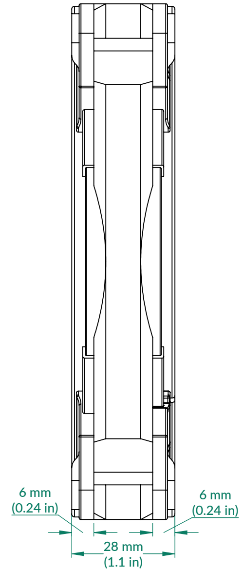
Side View
