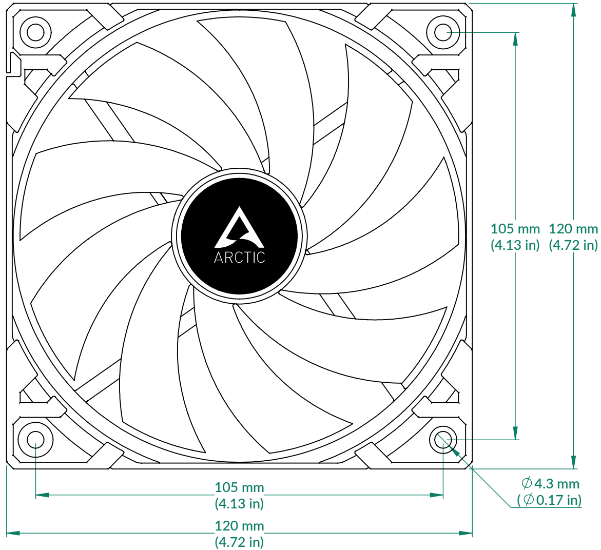
Front View
