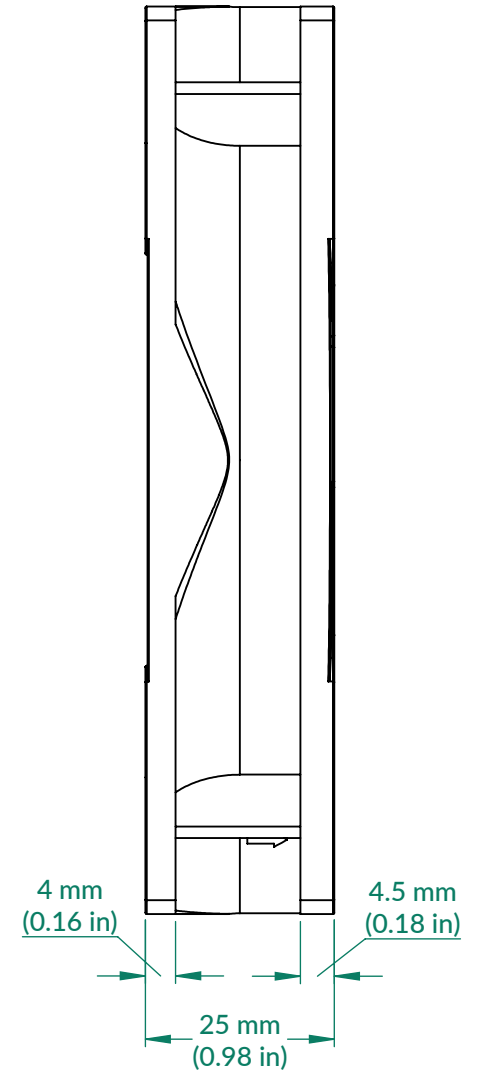
Side View
