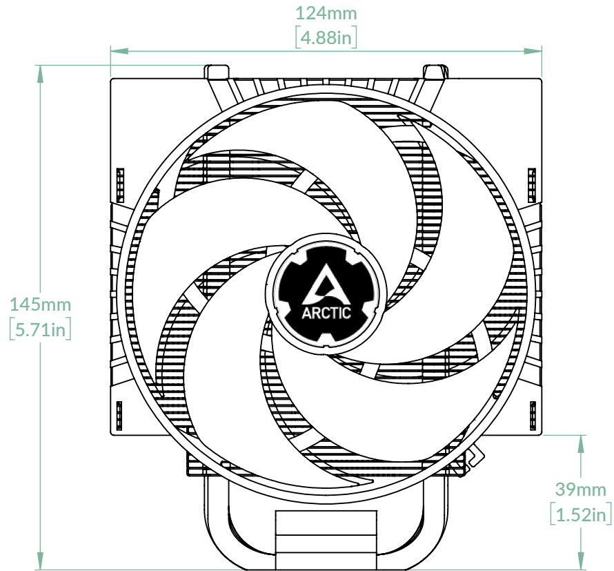
Front View
