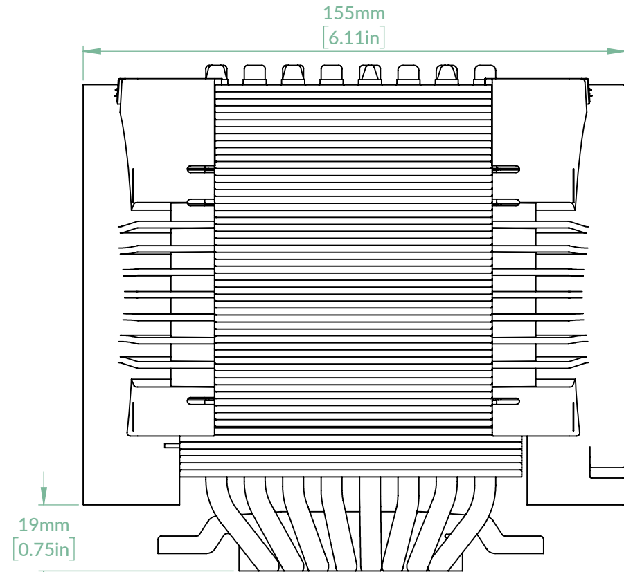
Side View
