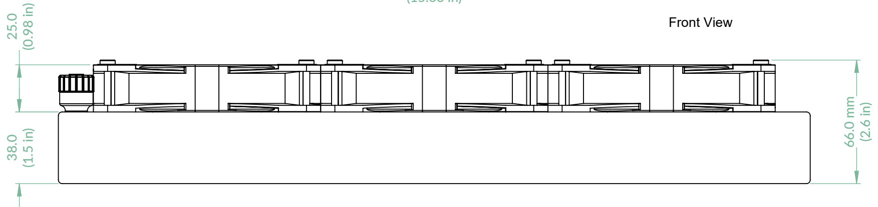
Side View
